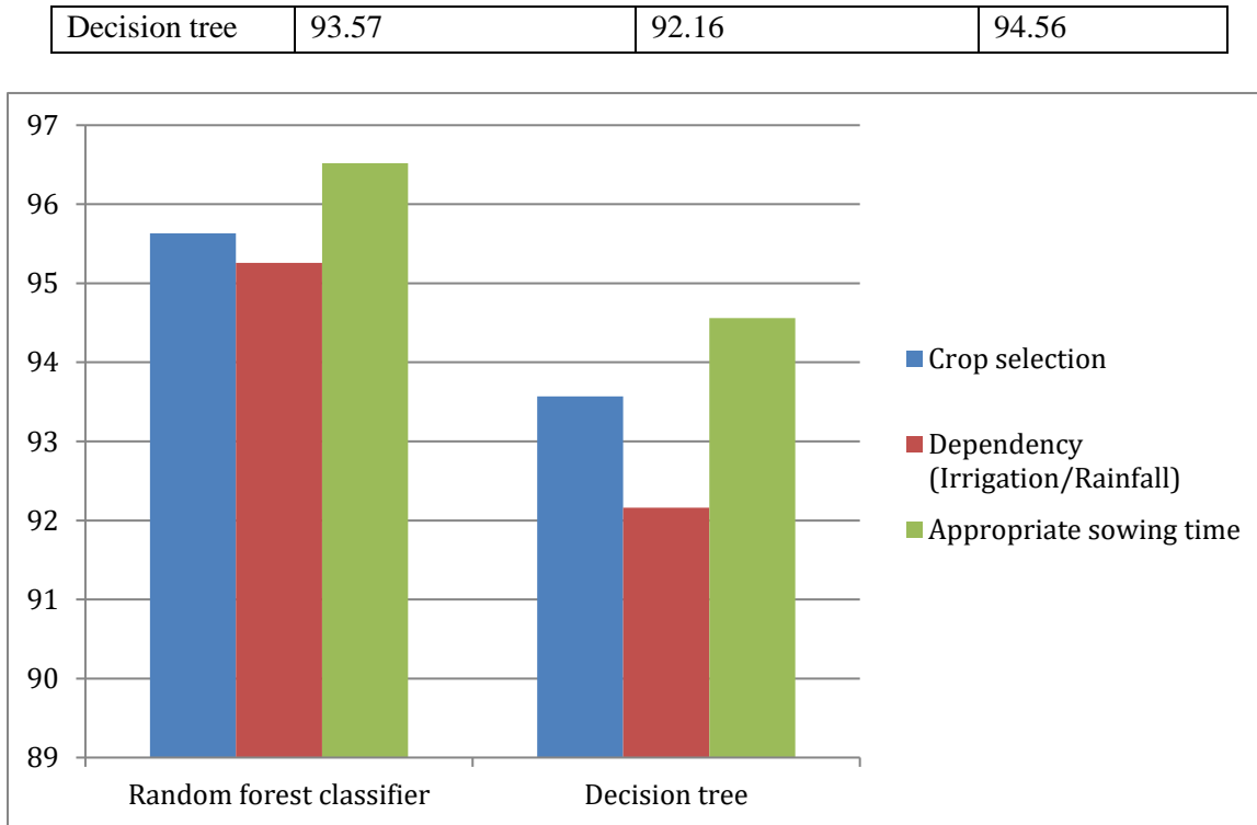
Figure 5: Accuracy Comparison
