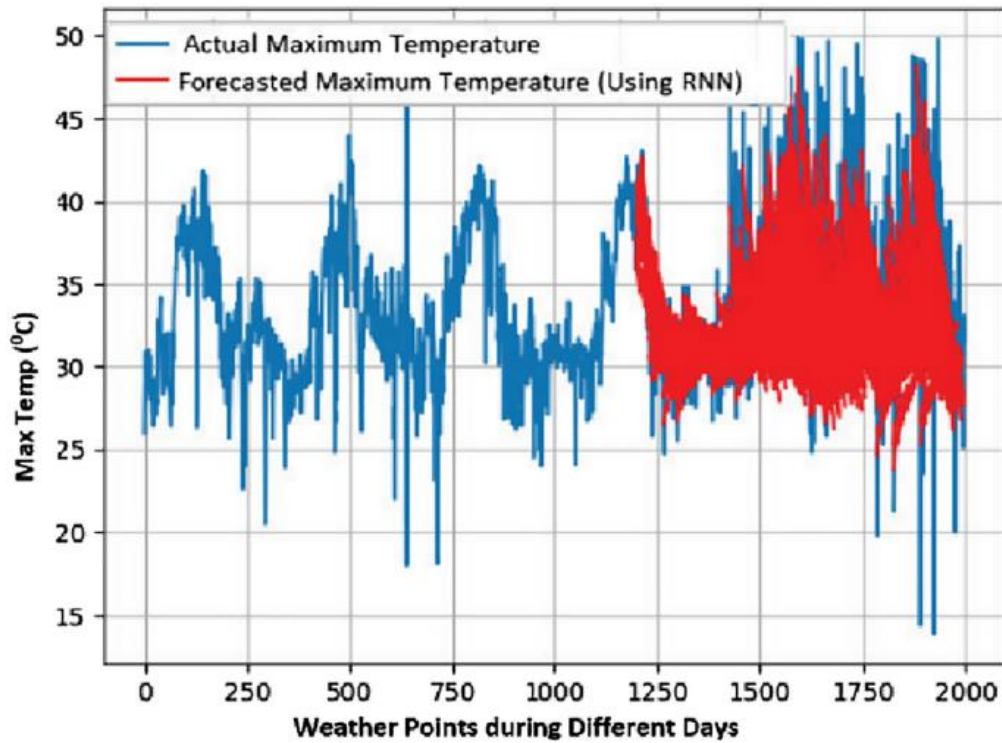
Figure 2: Maximum Temperature Prediction
