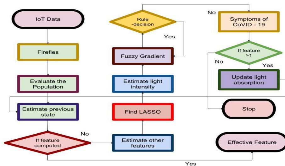
Figure 2: Feature Extraction and Selection
