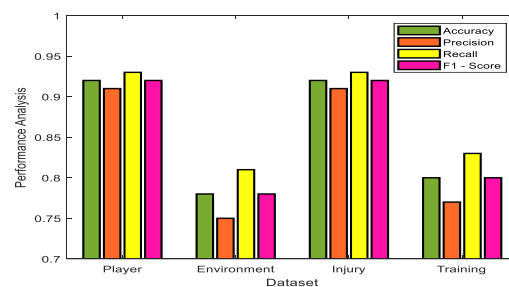
Figure 4: Performance Analysis of FfSGC
