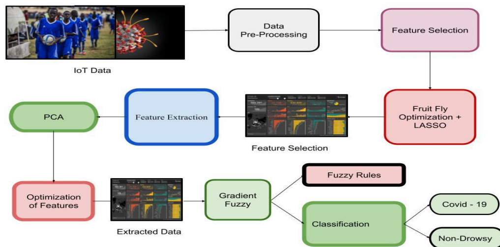
Figure 1: Architecture of FfSGC
