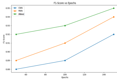
Figure 8: Comparison of F1-Score
