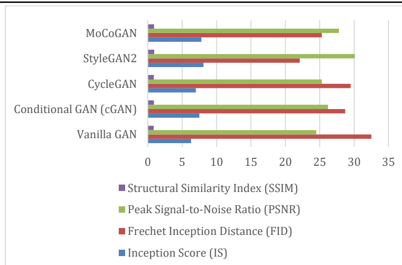
Figure 3: Performance of Different GAN
