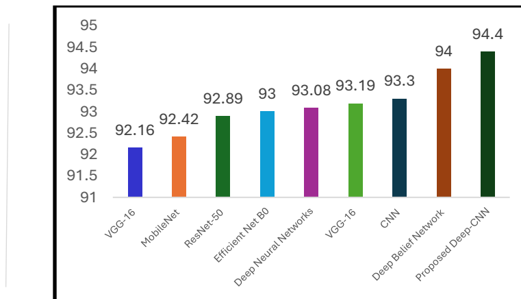
Figure7: Comparison of DEEP-CNN Model with state-of-the-art works
